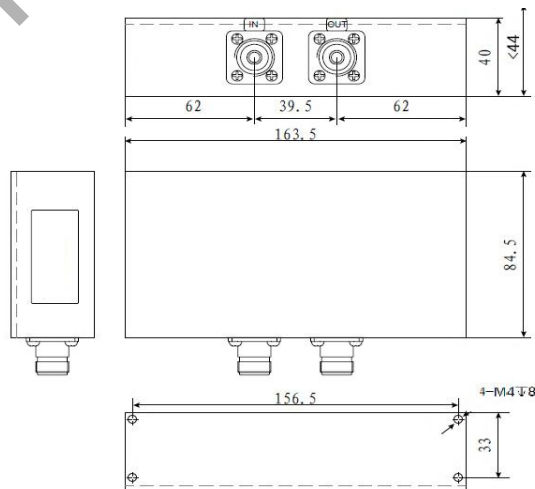
FILTER ONLY DIMENSIONS (mm)
